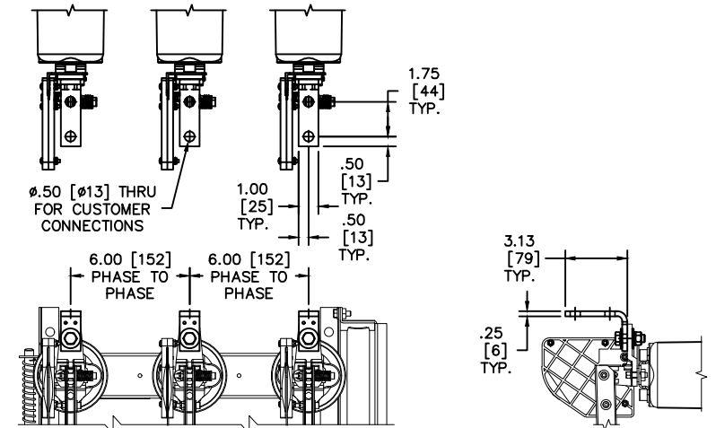
LINE SIDE LANDING PAD DETAIL "C"
