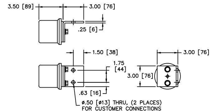
LANDING PAD DETAIL "B"
